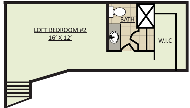
Plan D-1 2BR 2BA / 2nd FLOOR with LOFT TOTAL SQ. FT. 1,400
